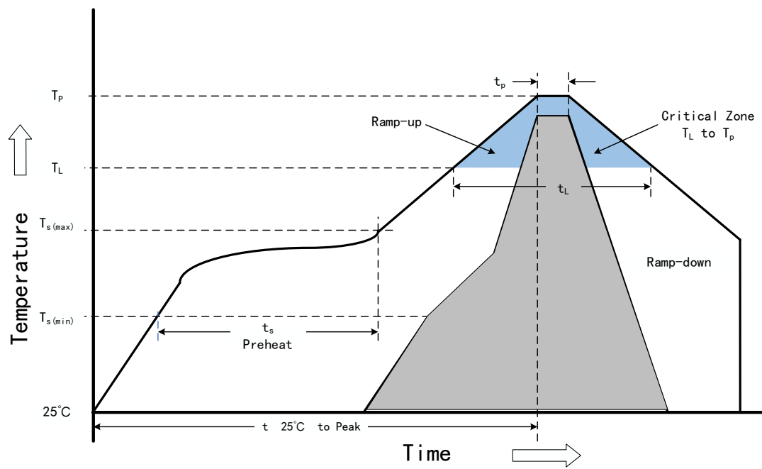
Fig 6.3 Soldering Profile
