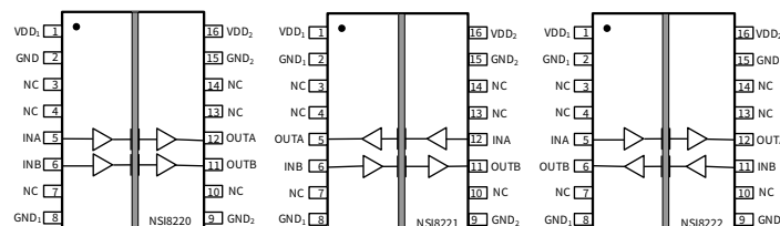
Figure 4. NSI822xWx SOWW16 Block Diagram
