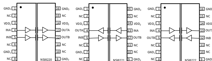
Figure 3. NSI822xWx SOW16 Block Diagram
