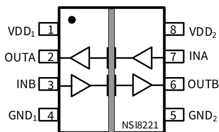
Figure 1.2 NSI8221N Package
