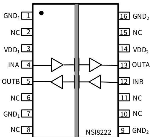
Figure 1.9 NSI8222W SOW16 Package
