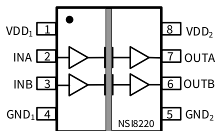
Figure 1.1 NSI8220N Package
