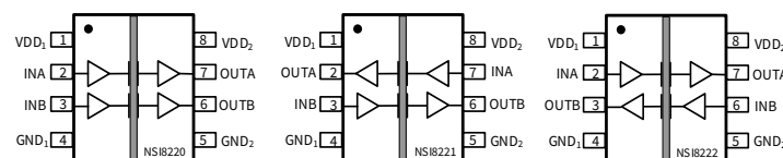
Figure 1. NSI822xNx SOP8 / NSI822xWx SOW8 Block Diagram
